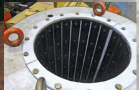
Main guide shaft bearing with ROMOR® I Rubber Staves
